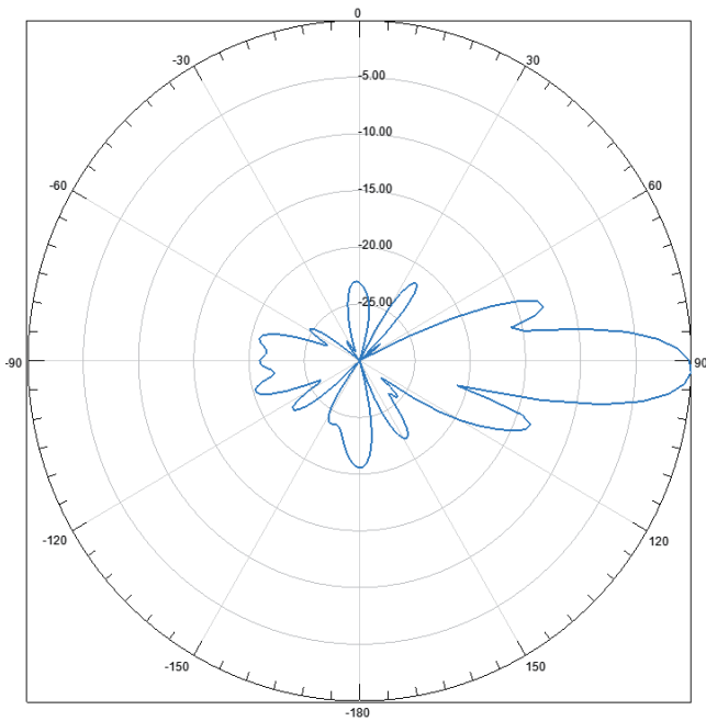
Vertical Elevation
